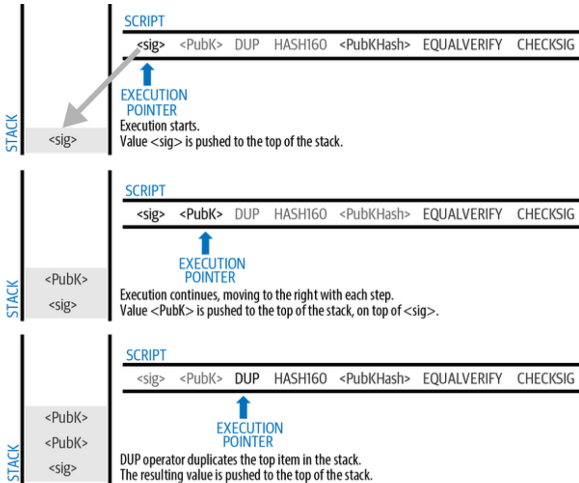
Figure 7-3. Evaluating a script for a P2PKH transaction (part 1 of 2).
