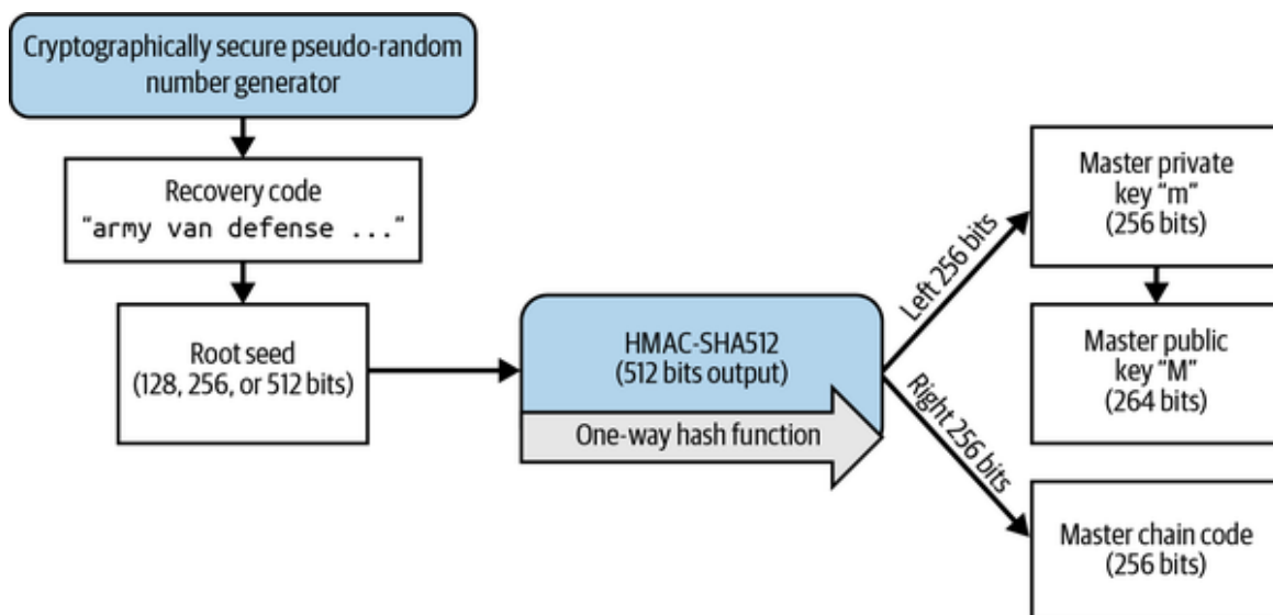
Figure 5-6. Creating master keys and chain code from a root seed.
