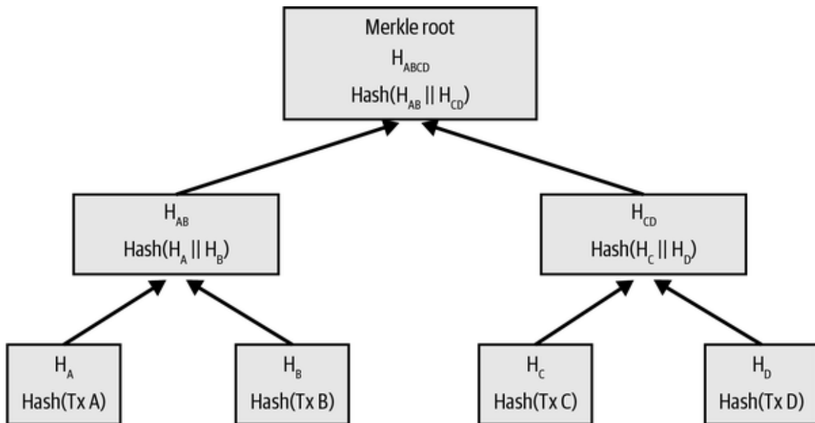
Figure 11-2. Calculating the nodes in a merkle tree.
