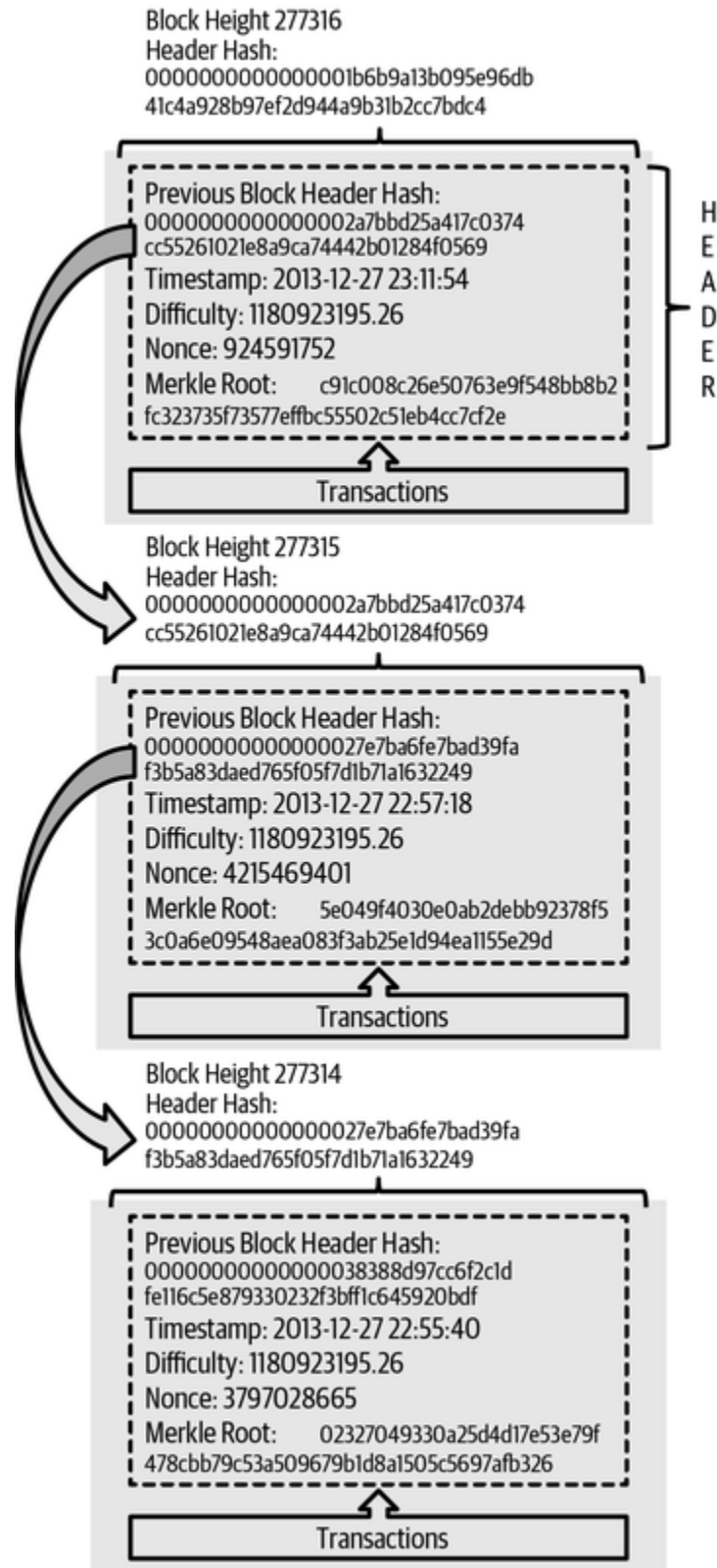
Figure 11-1. Blocks linked in a chain by each referencing the previous block header hash.
