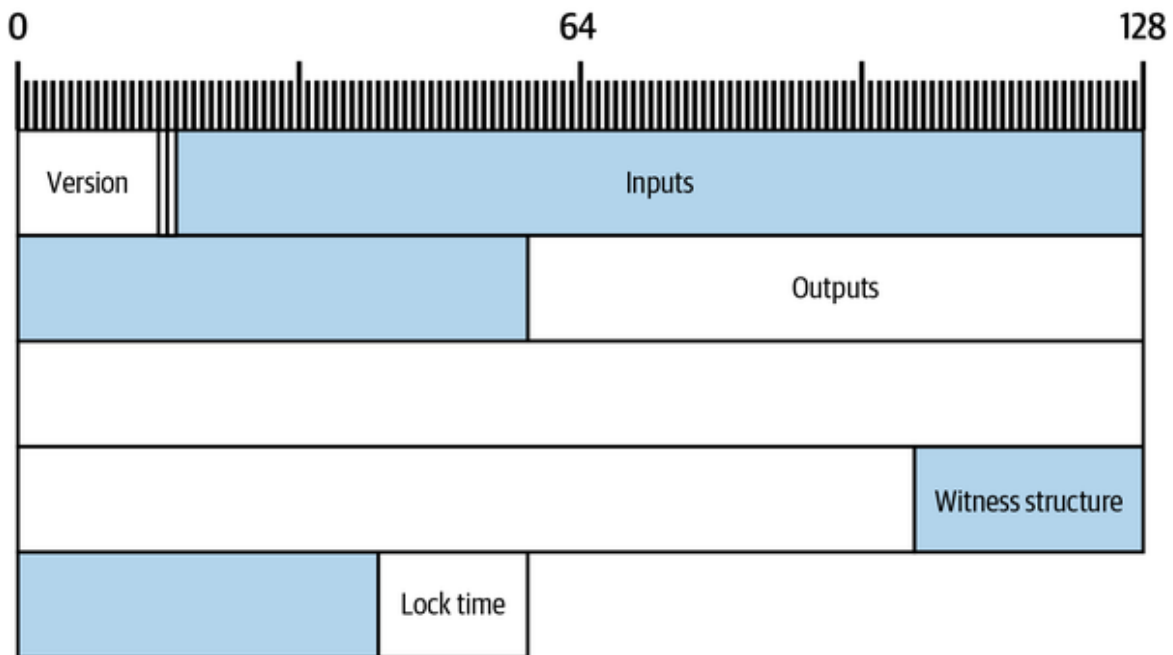
Figure 6-6. A byte map of Alice's transaction.
