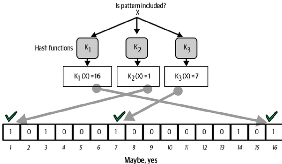
Figure 10-9. Testing the existence of pattern "X" in the bloom filter. The result is a probabilistic positive match, meaning "Maybe."
