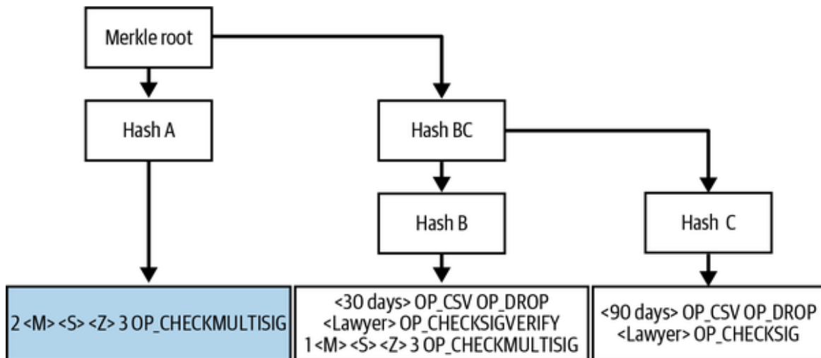
Figure 7-7. A MAST with the most-expected script in the best position.
