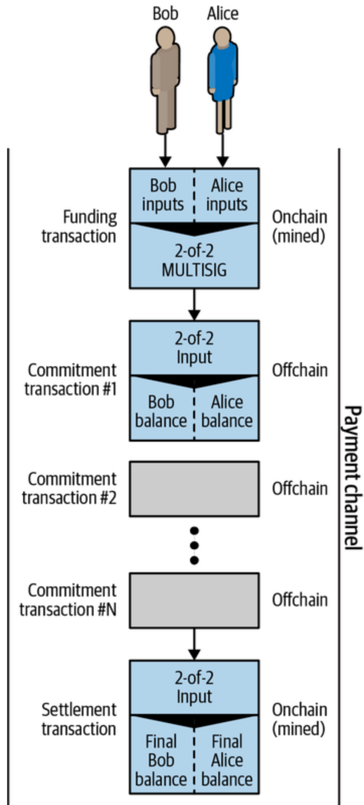
Figure 14-1. A payment channel between Bob and Alice, showing the funding, commitment, and settlement transactions.
