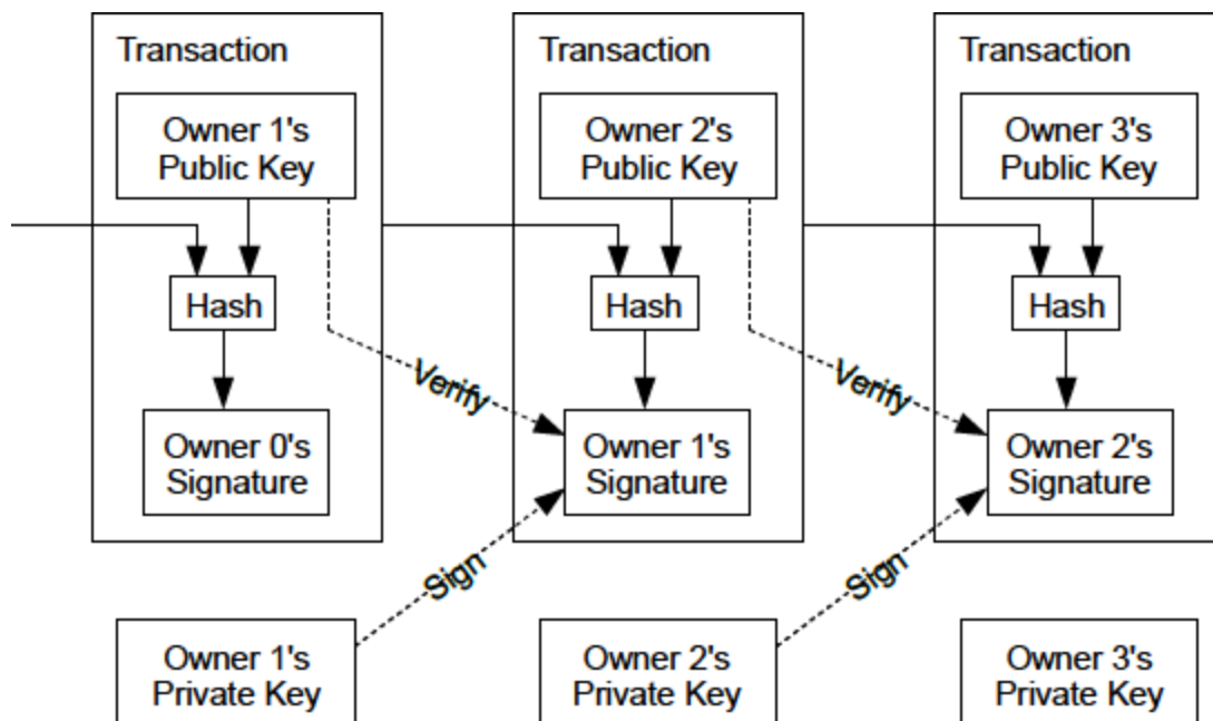
Figure 4-1. Transaction chain from original Bitcoin paper.
