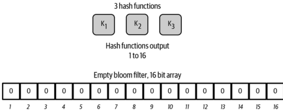
Figure 10-6. An example of a simplistic bloom filter, with a 16-bit field and three hash functions.
