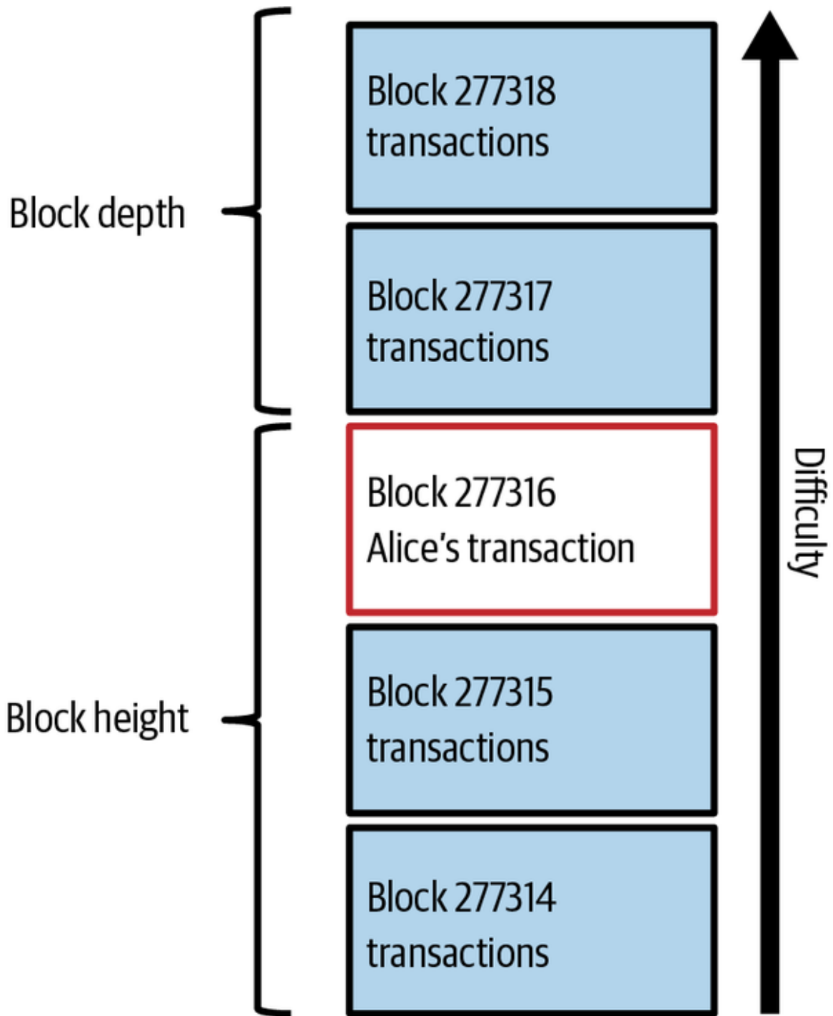
Figure 2-7. Alice's transaction included in a block.
