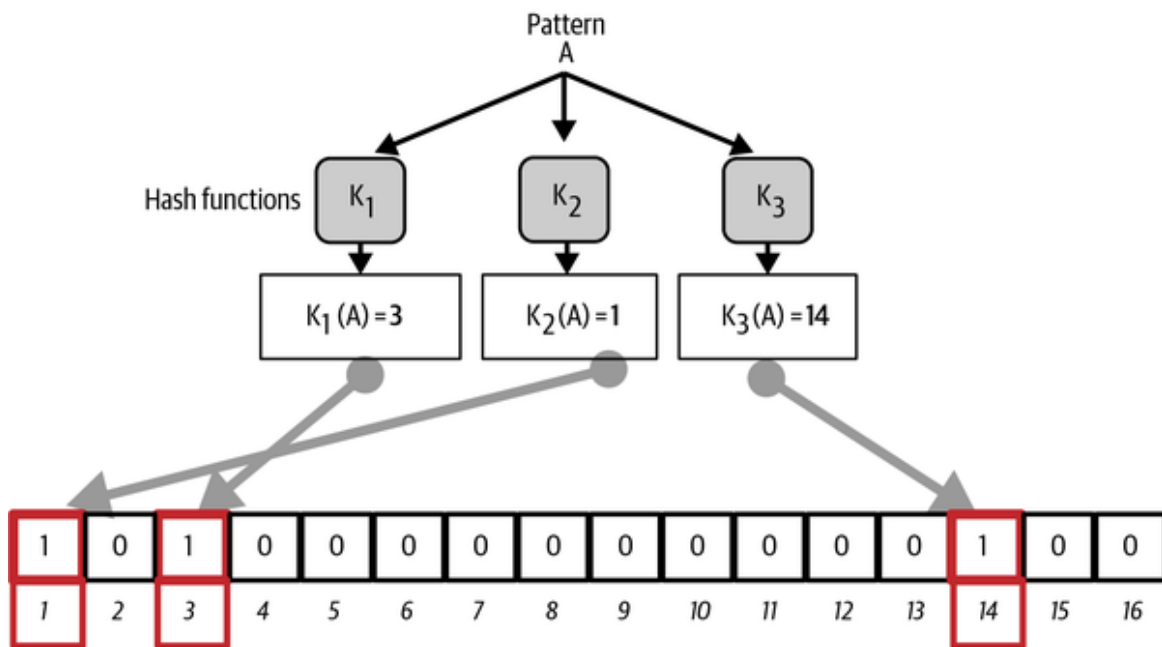
Figure 10-7. Adding a pattern "A" to our simple bloom filter.
