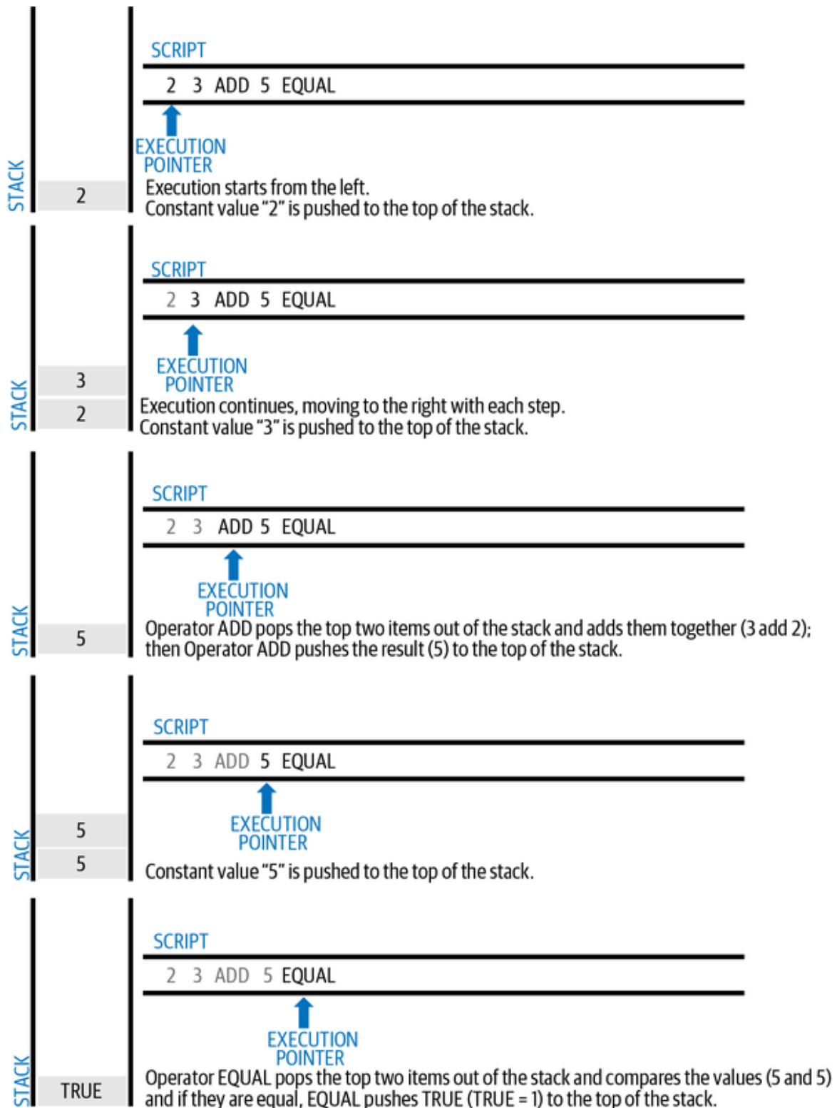
Figure 7-2. Bitcoin's script validation doing simple math.
