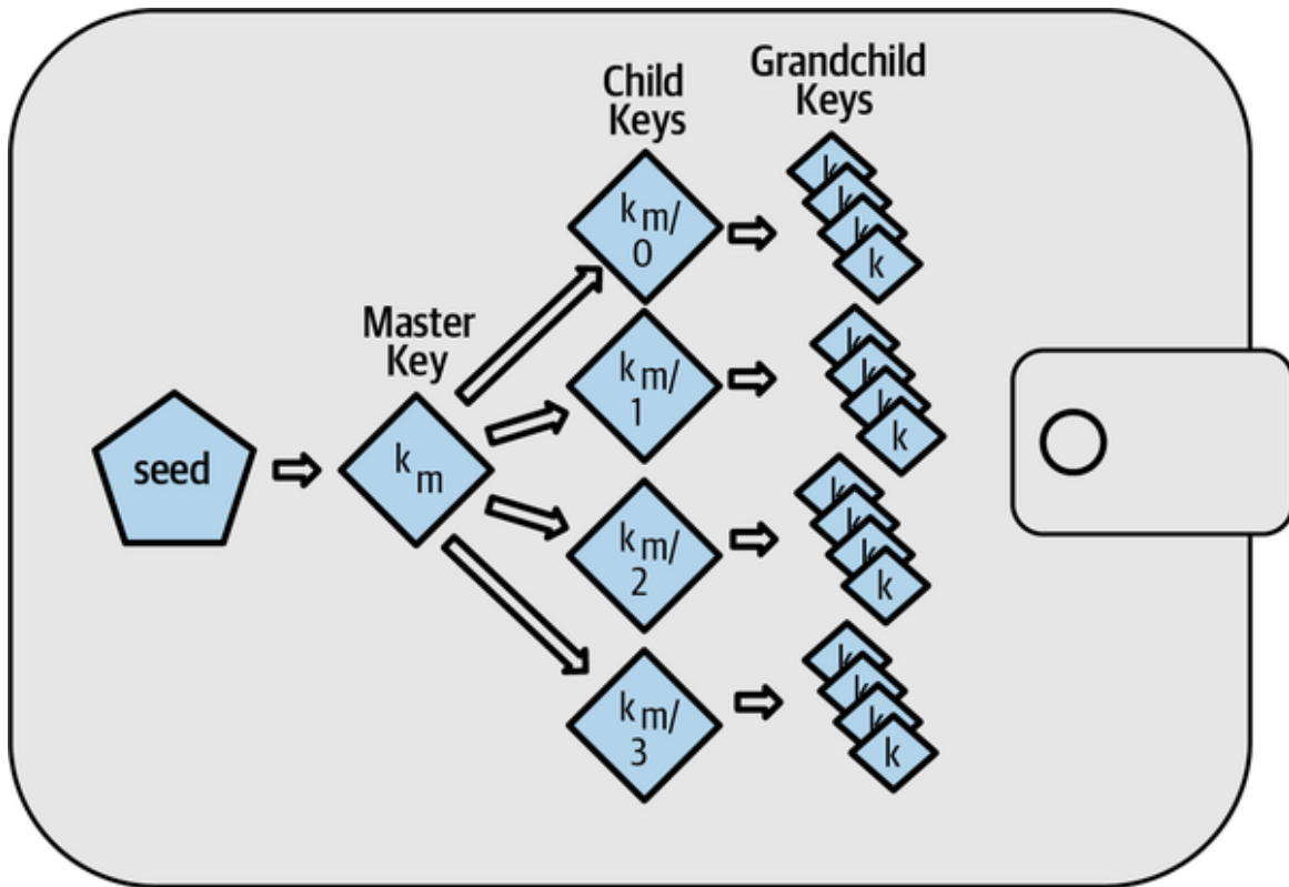
Figure 5-3. HD wallet: a tree of keys generated from a single seed.
