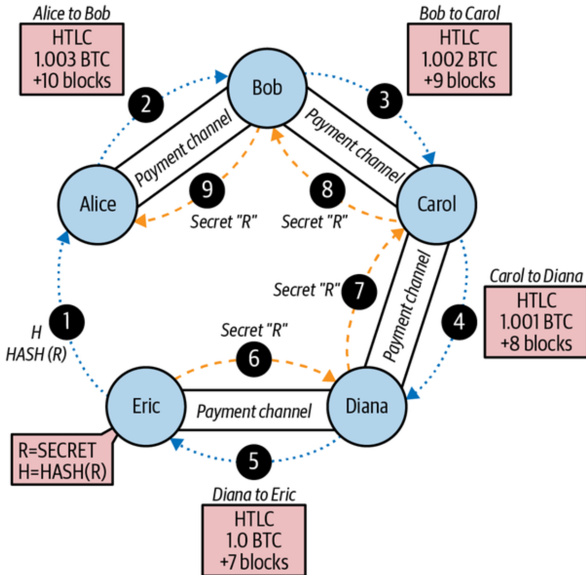
Figure 14-7. Step-by-step payment routing through an LN.
