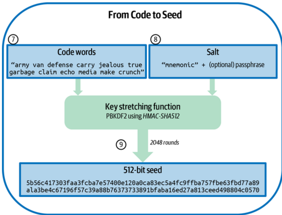
Figure 5-5. From recovery code to seed.
