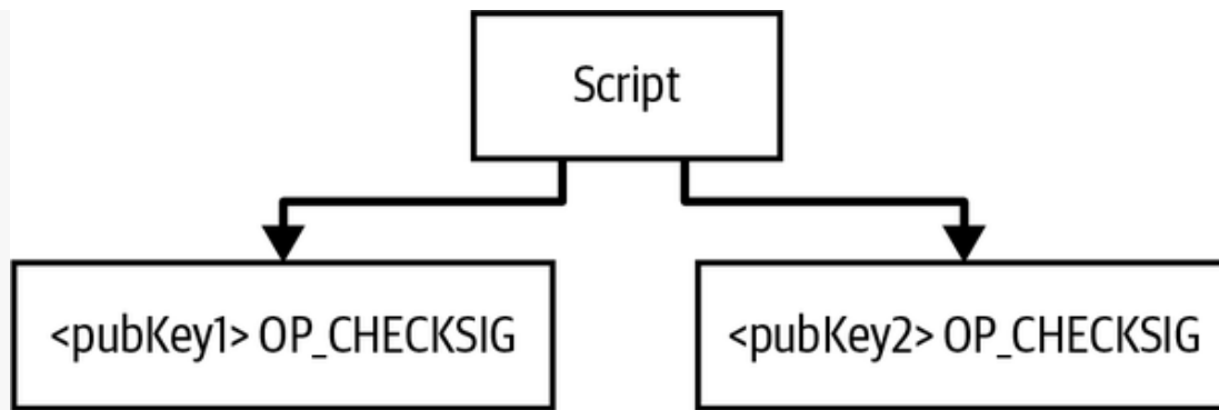
Figure 7-9. An alternative script tree.
