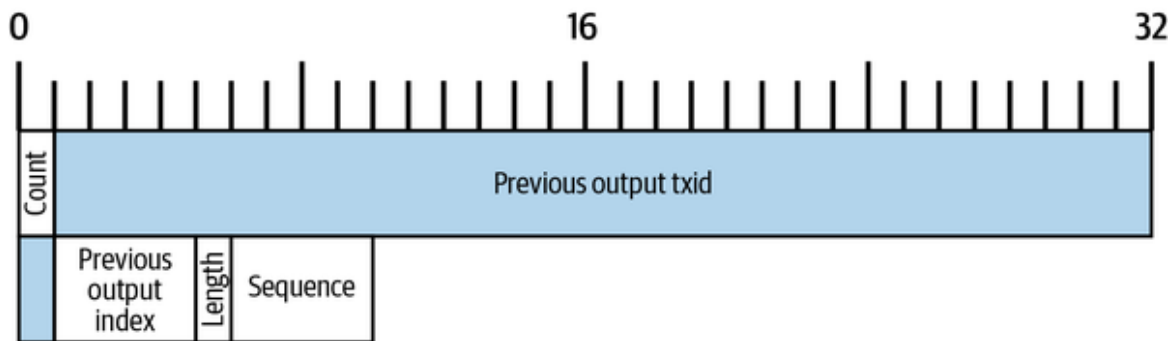
Figure 6-2. Map of bytes in the inputs field of Alice’s transaction.
