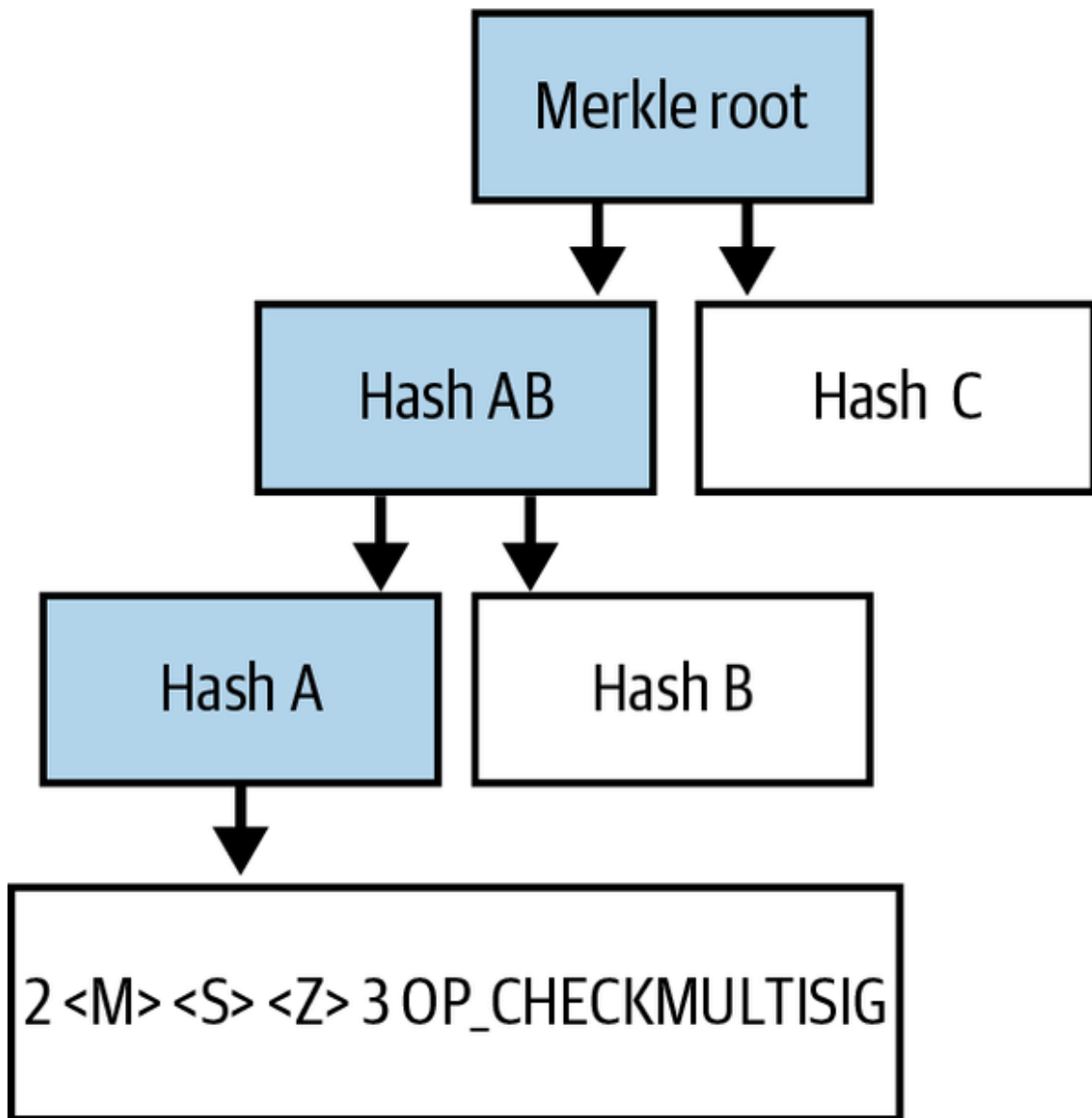
Figure 7-6. A MAST membership proof for one of the subscripts.
