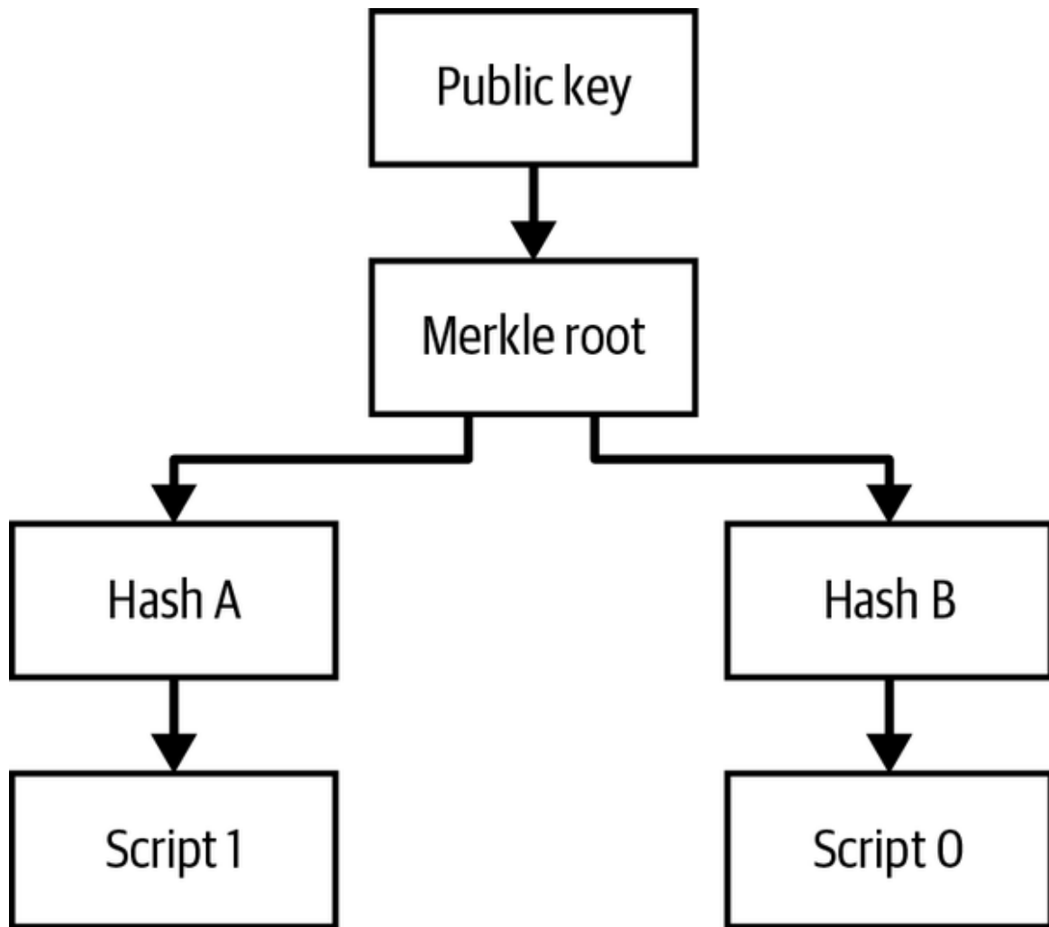
Figure 7-10. A taproot with the public key committing to a merkle root.
