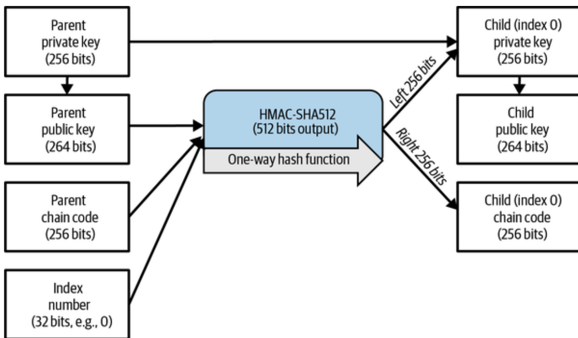
Figure 5-7. Extending a parent private key to create a child private key.
