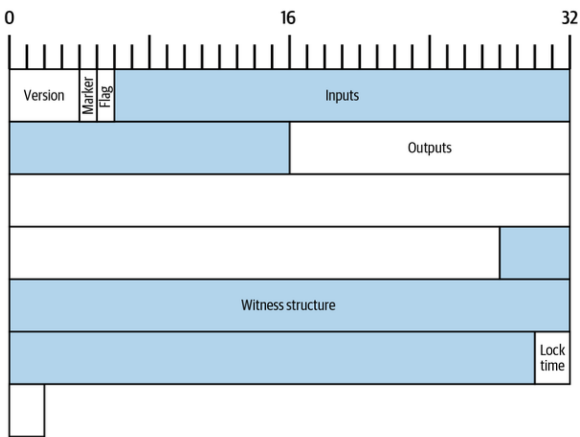
Figure 6-1. A byte map of Alice’s transaction.
