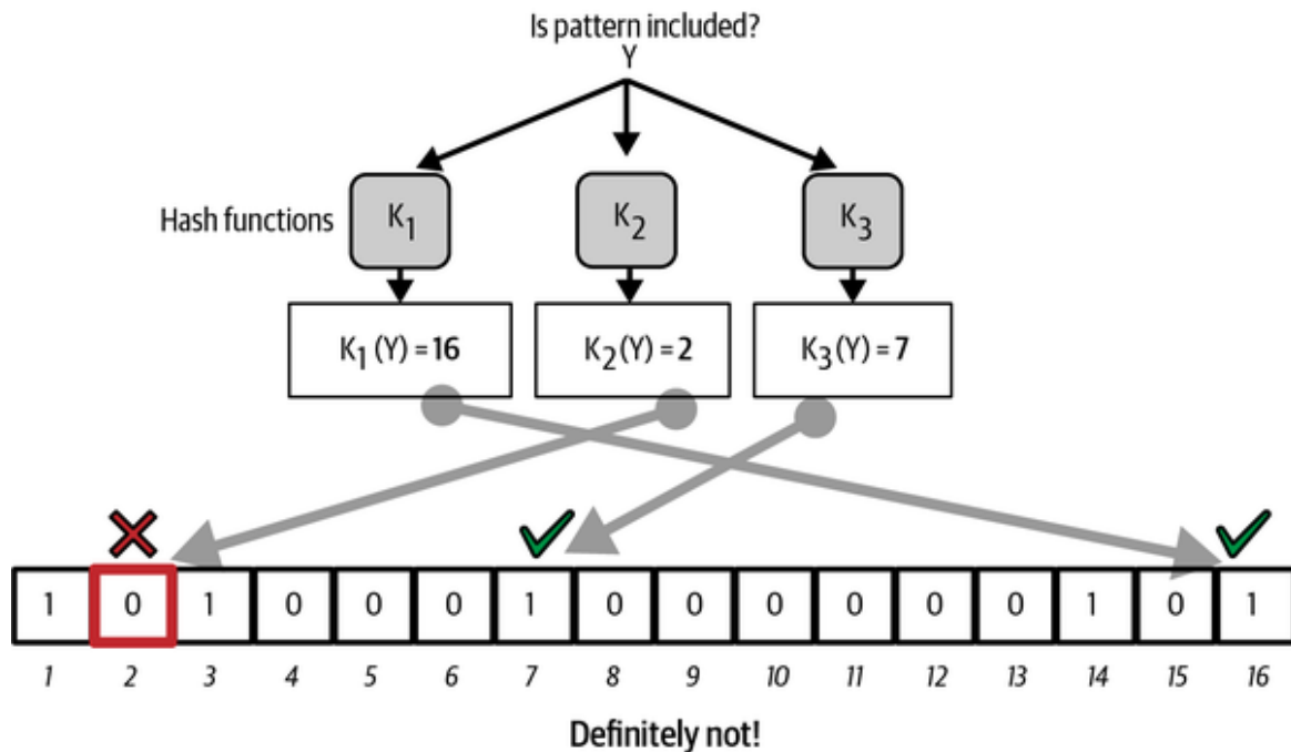
Figure 10-10. Testing the existence of pattern “Y” in the bloom filter. The result is a definitive negative match, meaning “Definitely Not!”
