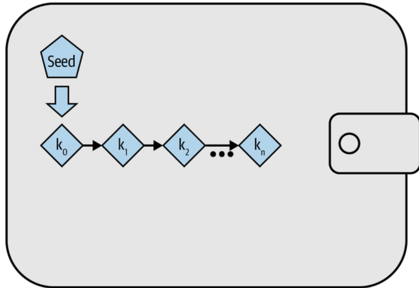
Figure 5-2. Deterministic key generation: a deterministic sequence of keys derived from a seed for a wallet database.
