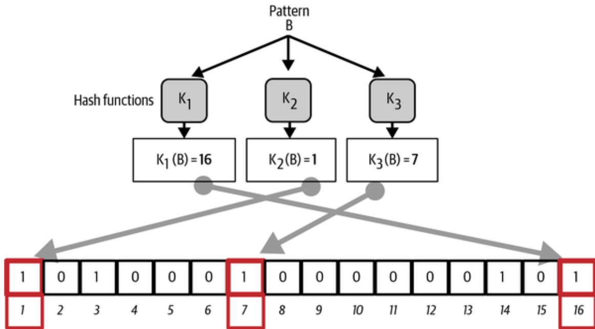
Figure 10-8. Adding a second pattern "B" to our simple bloom filter.
