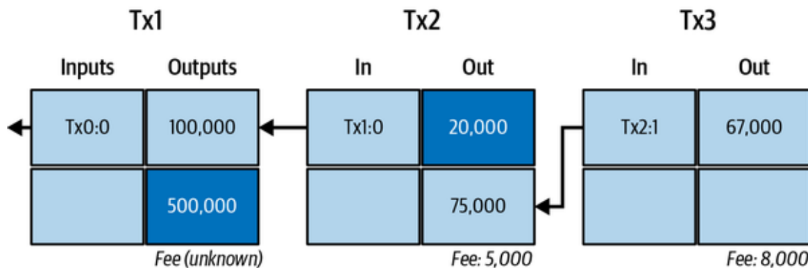
Figure 2-3. A chain of transactions, where the output of one transaction is the input of the next transaction.
