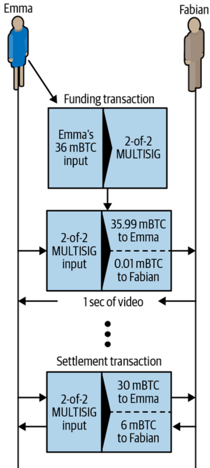
Figure 14-3. Emma's payment channel with Fabian, showing the commitment transactions that update the balance of the channel.
