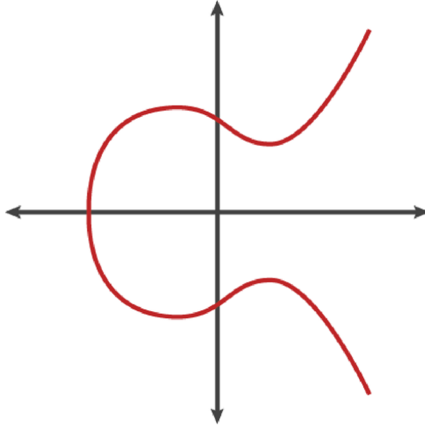
Figure 4-2. An elliptic curve.
