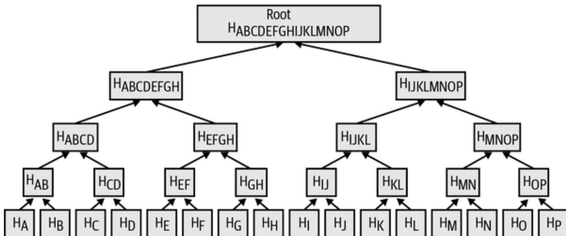
Figure 11-5. A merkle tree summarizing many data elements.
