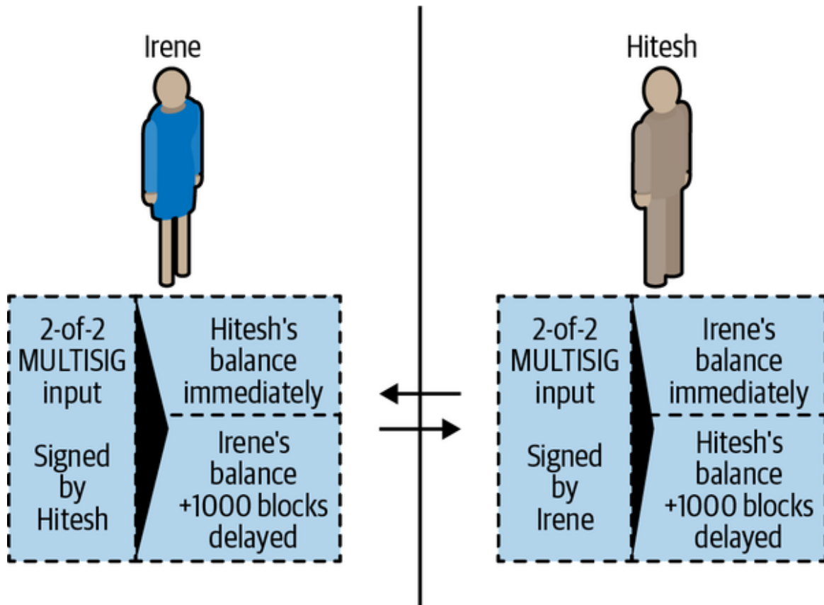
Figure 14-5. Two asymmetric commitment transactions with delayed payment for the party holding the transaction.
