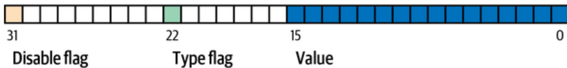
Figure 6-3. BIP68 definition of sequence encoding (Source: BIP68).
