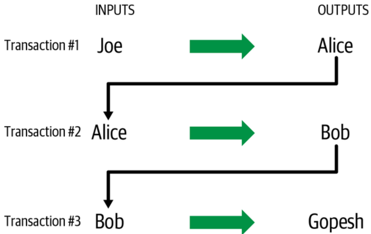
Figure 2-8. Alice's transaction as part of a transaction chain from Joe to Gopesh.
