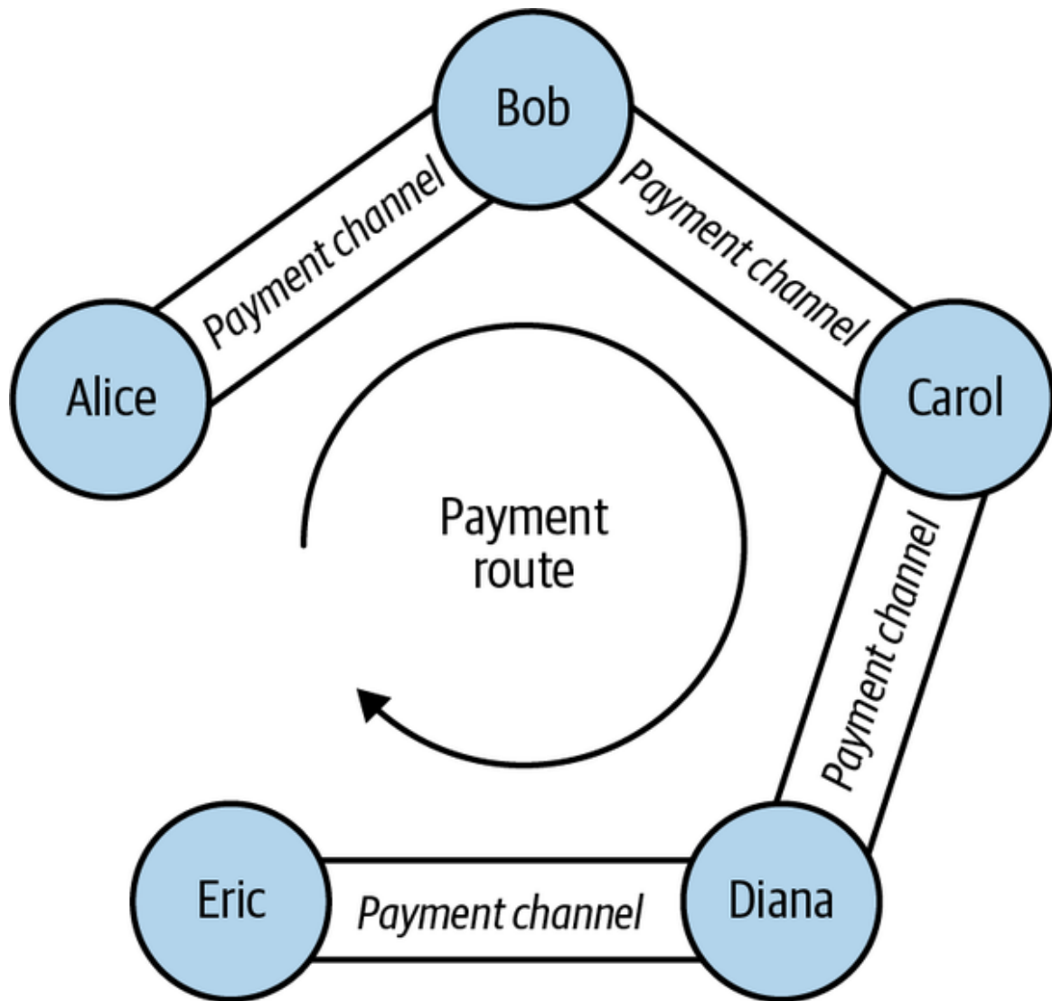
Figure 14-6. A series of bidirectional payment channels linked to form an LN that can route a payment from Alice to Eric.
