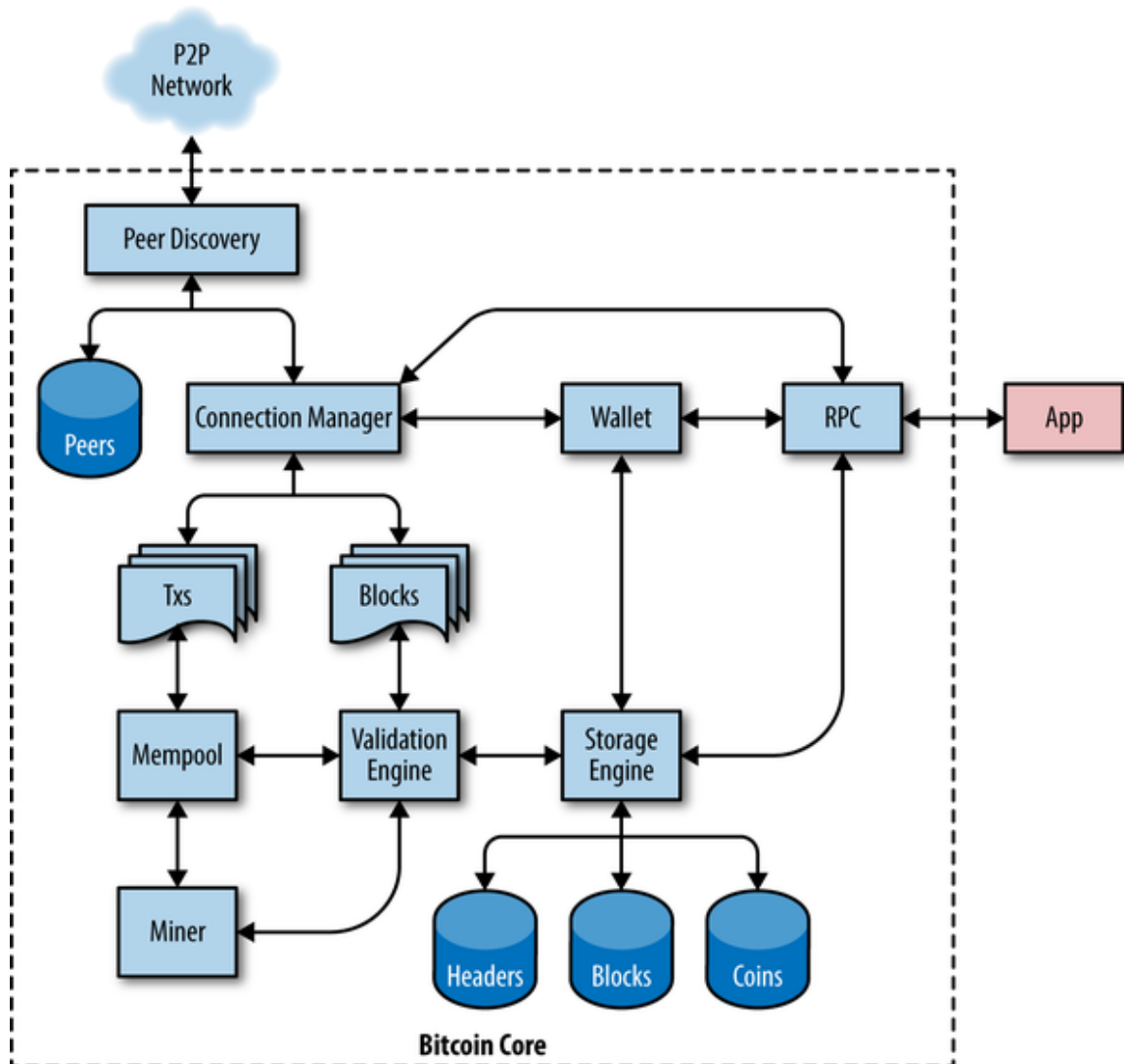
Figure 3-1. Bitcoin Core architecture (Source: Eric Lombrozo).
