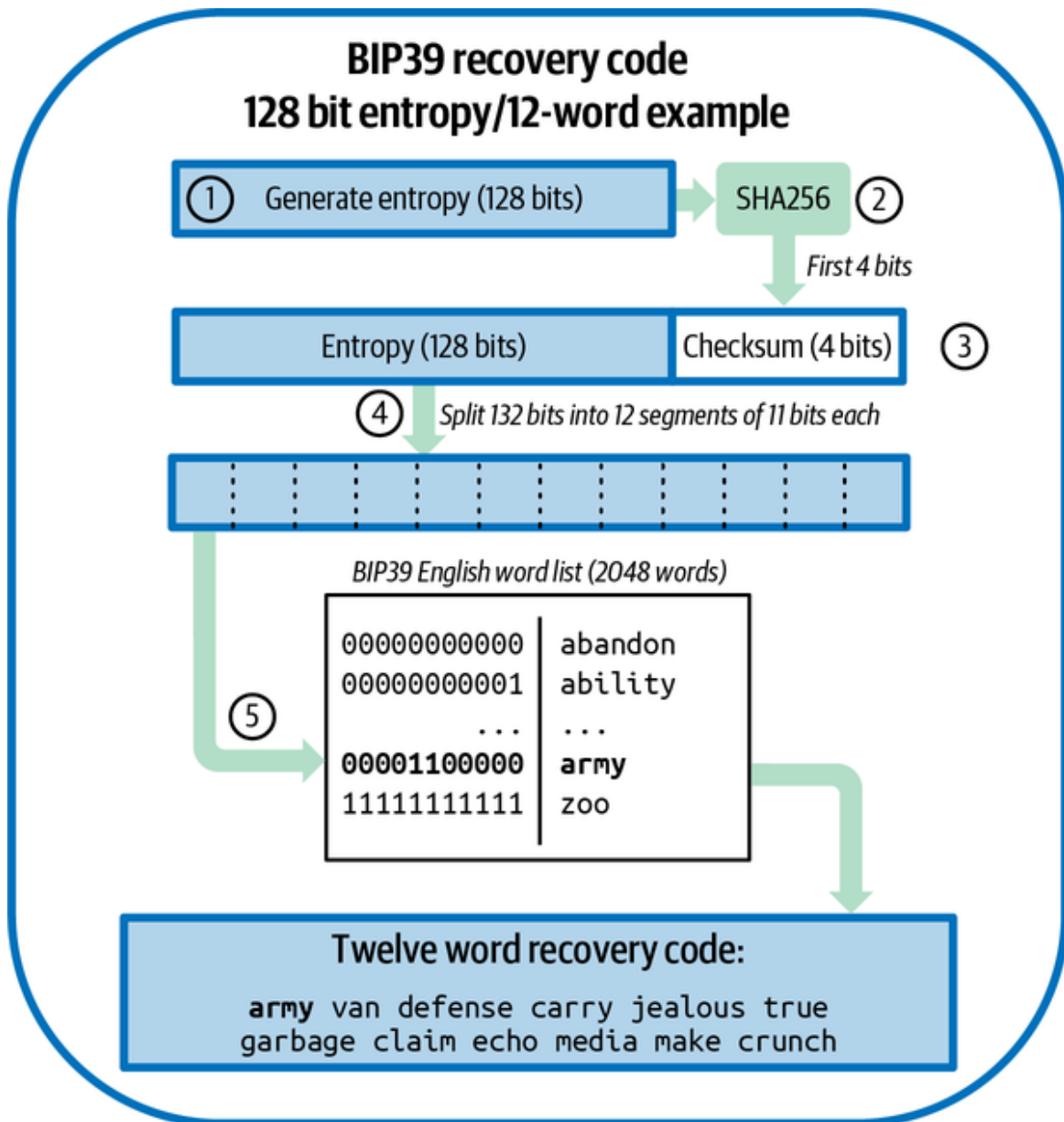
Figure 5-4. Generating entropy and encoding as a recovery code.
