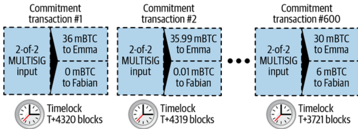
Figure 14-4. Each commitment sets a shorter timelock, allowing it to be spent before the previous commitments become valid.
