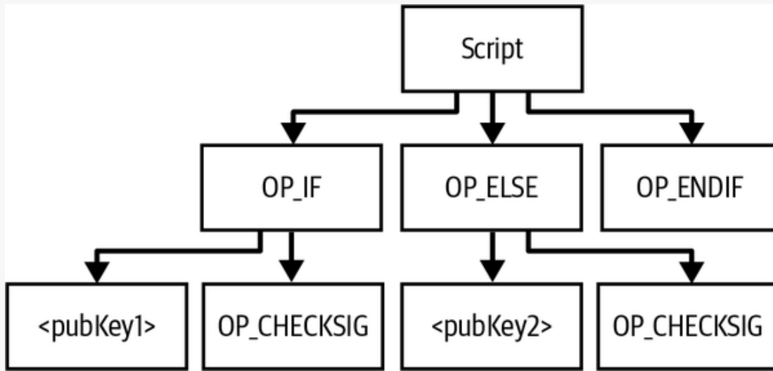
Figure 7-8. An abstract syntax tree (AST) for a script.
