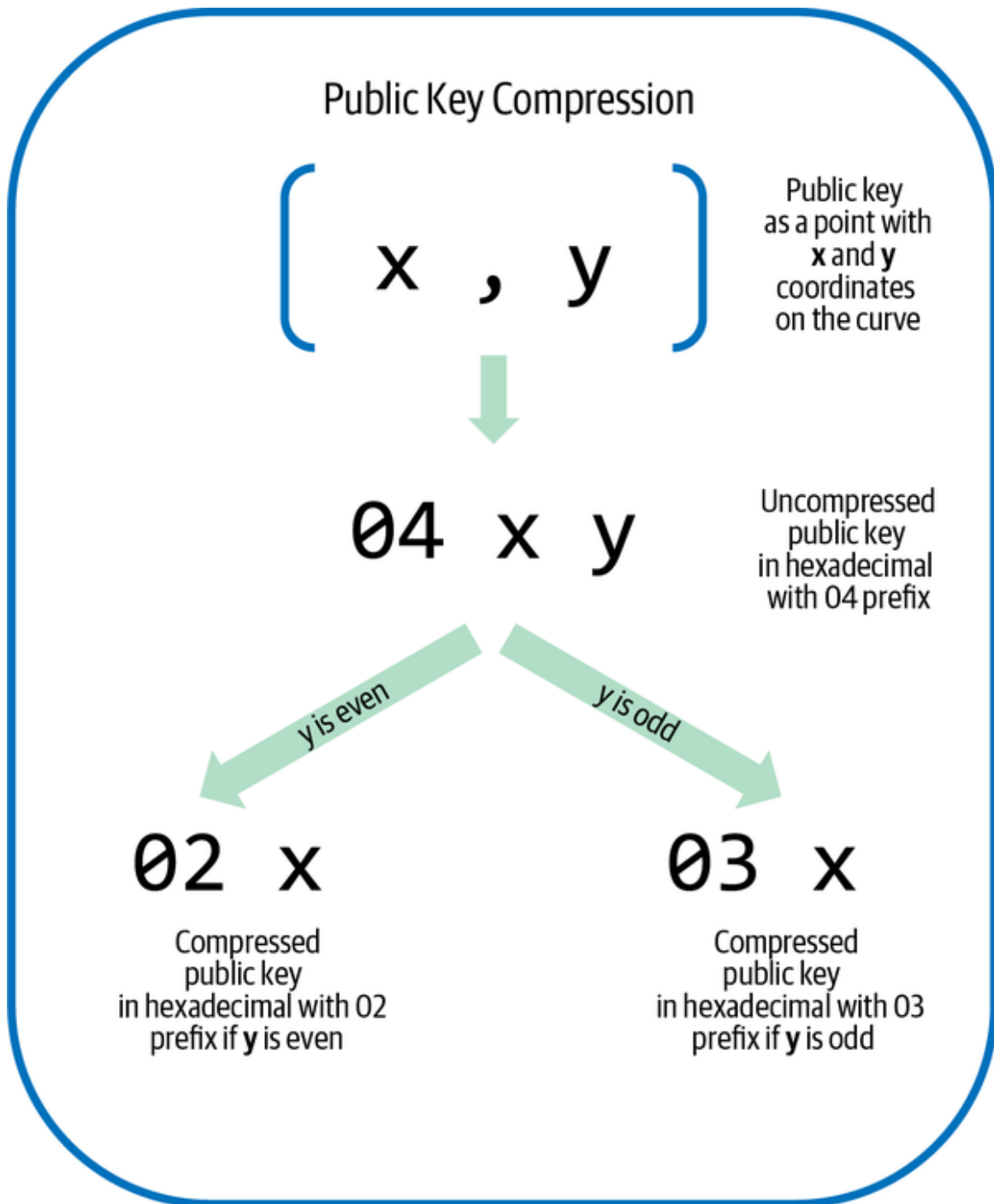
Figure 4-8. Public key compression.
