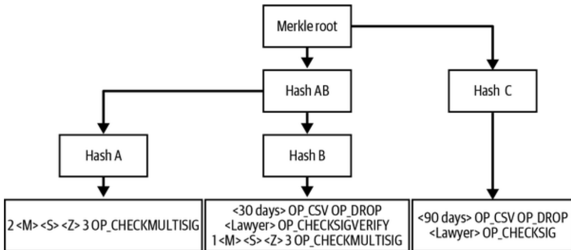
Figure 7-5. A MAST with three subscripts.
