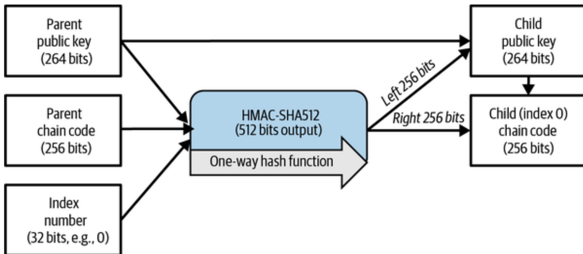
Figure 5-8. Extending a parent public key to create a child public key.
