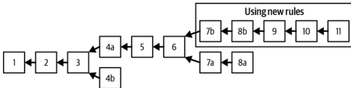
Figure 12-2. A blockchain with forks.
