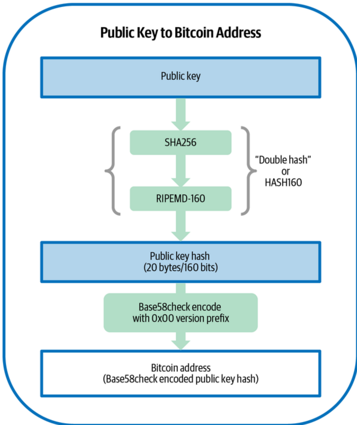
Figure 4-7. Public key to Bitcoin address: conversion of a public key to a Bitcoin address.
