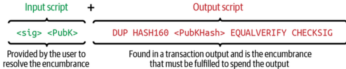
Figure 7-1. Combining input and output scripts to evaluate a transaction script.
