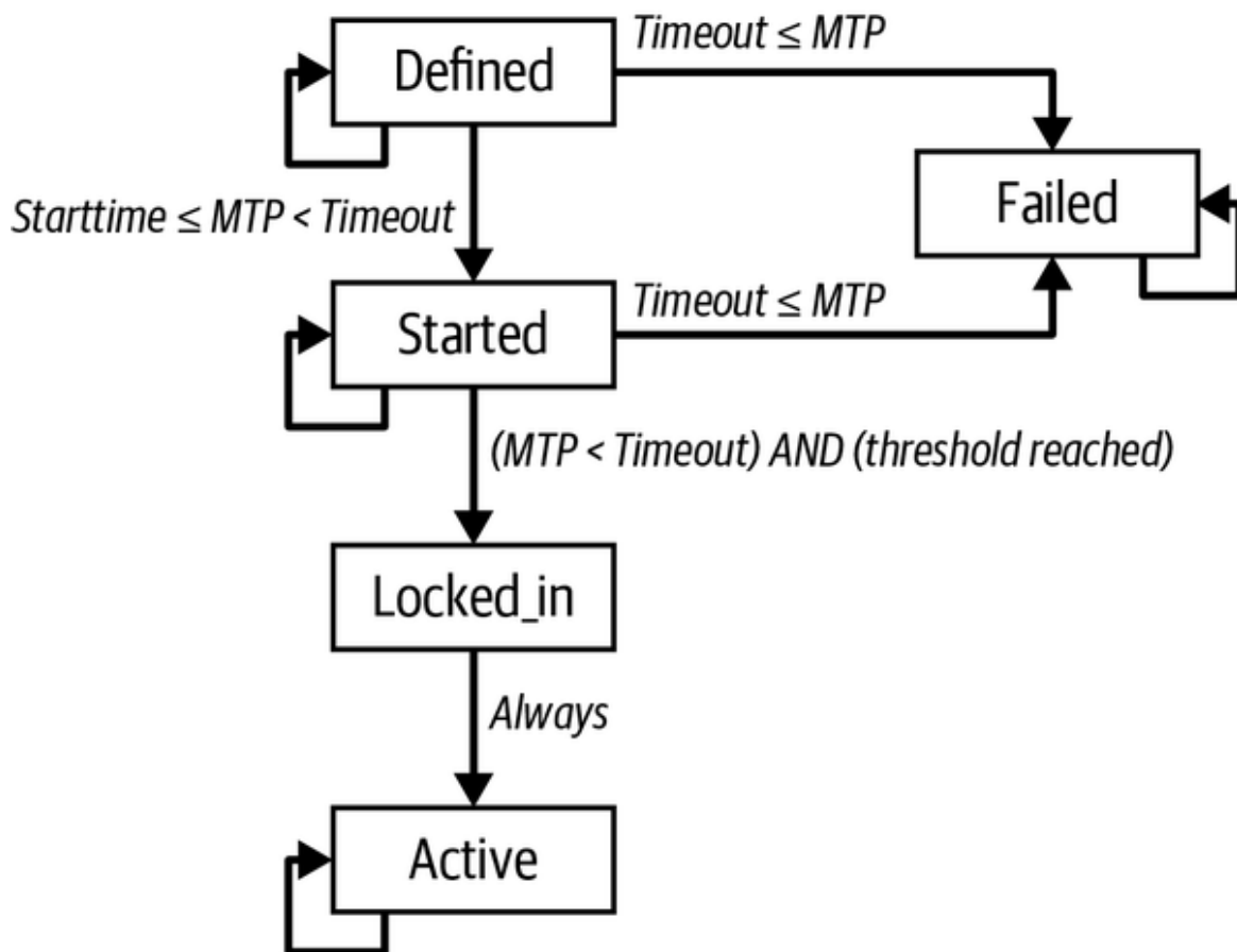
Figure 12-3. BIP9 state transition diagram.
